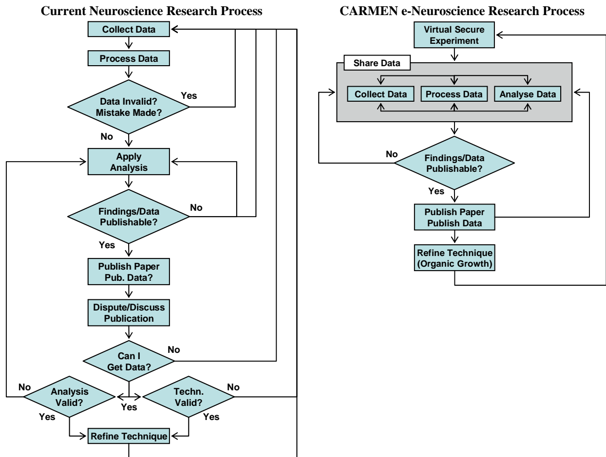
Figure 2: Current Neuroscience Research Process vs CARMEN Neuroscience Research Process
