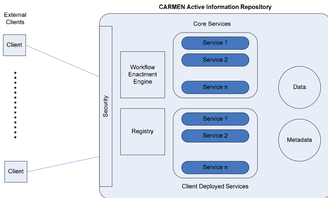
Figure 3: A CARMEN Active Information Repository Node (CAIRN)
